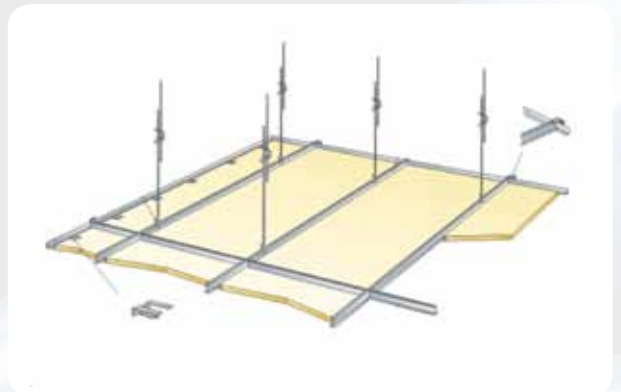
Quick Suspension system / System 2000
